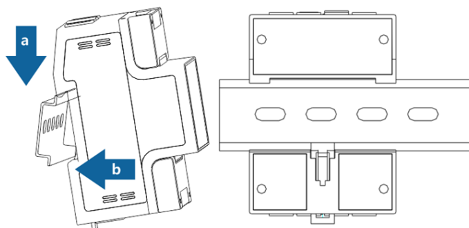
Figure9 install picture
