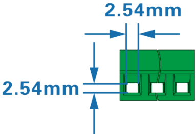
Figure7 current cable terminal (Conductor Cross-sectional Area Range ≤16 mm 2 )
