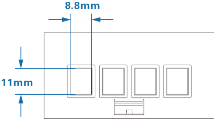
Figure7 current cable terminal (Conductor Cross-sectional Area Range ≤16 mm 2 )
